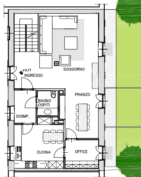
GROUND FLOOR mq 97
