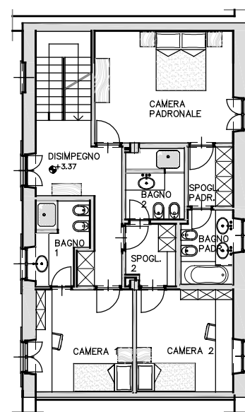
FIRST FLOOR mq 97
