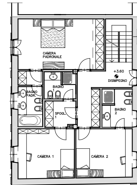
FIRST FLOOR mq 106
